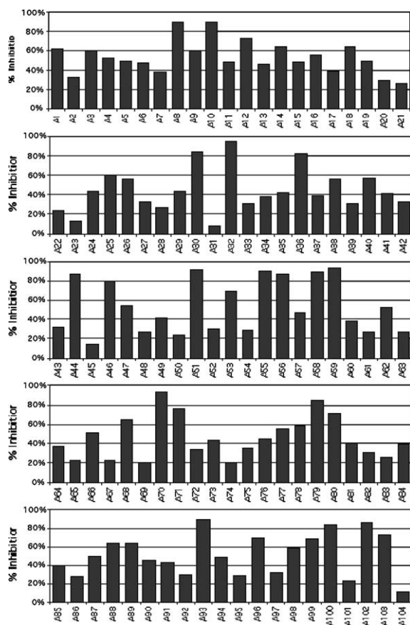
Figure 3. Assay of library members at 1 \mu M concentration against the Yersinia PTPase. Designators on the x-axis refer to the library members shown in Figure 2.
