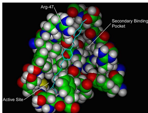
Figure 1. Computer generated model of compound 2 bound in the active site of PTP1B.
