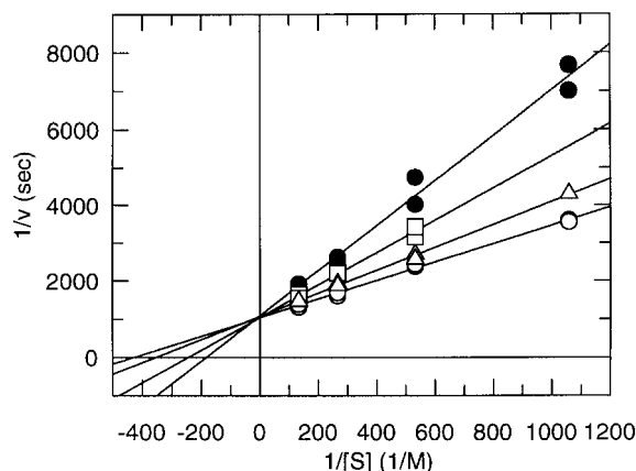
Figure 5. Inhibition of PTP1B by compound 14 . The activity of PTP1B was measured at pH 7.0 as described under the Experimental Section in the presence of the following concentrations of 14 : (○) 0 \mu M; ( \Delta ) 1.27 \mu M; ( \square ) 2.54 \mu M; ( \bullet ) 3.80 \mu M. Substrate concentrations used in the assays were 0.94, 1.88, 3.76, and 7.53 mM.
