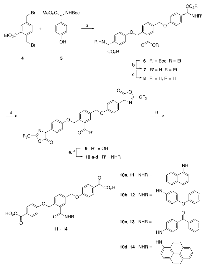
Scheme 1. Reagents and conditions: (a) Na, EtOH, 90%; (b) TFA, CH 2 Cl 2 , 91%; (c) NaOH, H 2 O; (d) trifluoroacetic anhydride, 76% (two steps); (e) SOCl 2 , benzene; (f) RNH 2 , CH 2 Cl 2 or THF; (g) NaOH, H 2 O.
