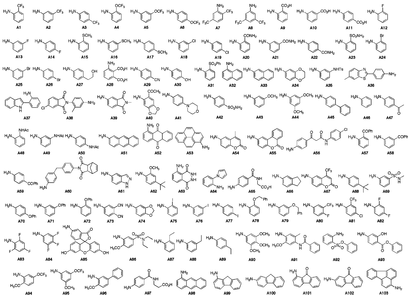
Figure 2. Aromatic amines used to synthesize the library. The designator under each aromatic amine refers to the library member with general structure 3 where the R component is derived from the above amines.
