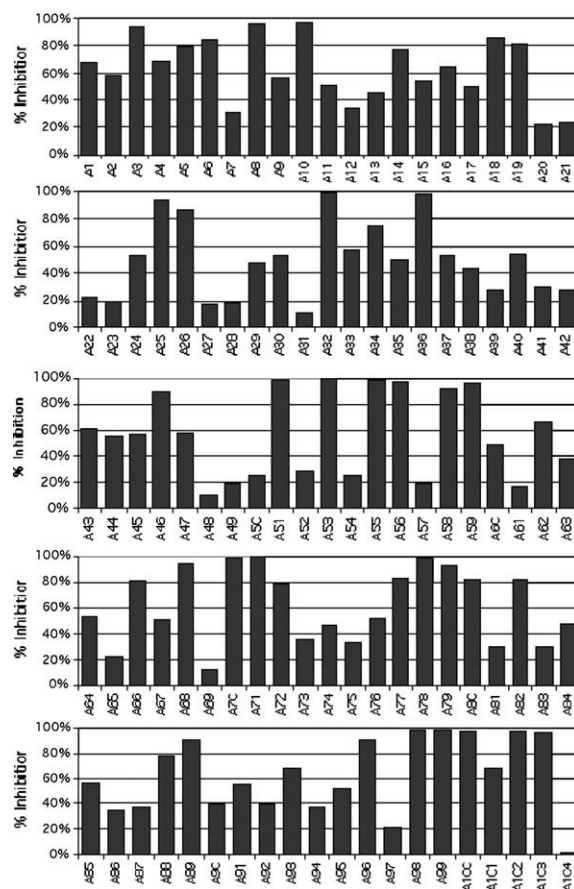
Figure 4. Assay of library members at 5 \mu M concentration against PTP1B. Designators on the x-axis refer to the library members shown in Figure 2.
